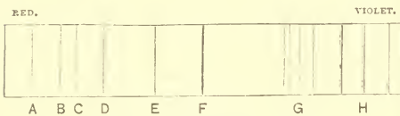
Fig. 4.—Solar Absorption Lines.
